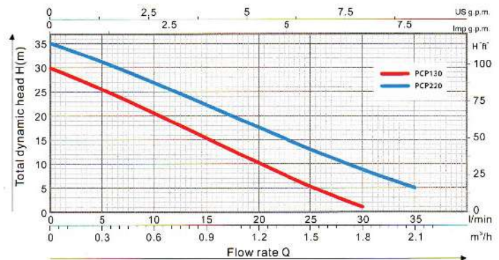
Performance Chart at n=2850 r/min
