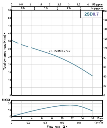
PERFORMANCE DATA 50Hz
